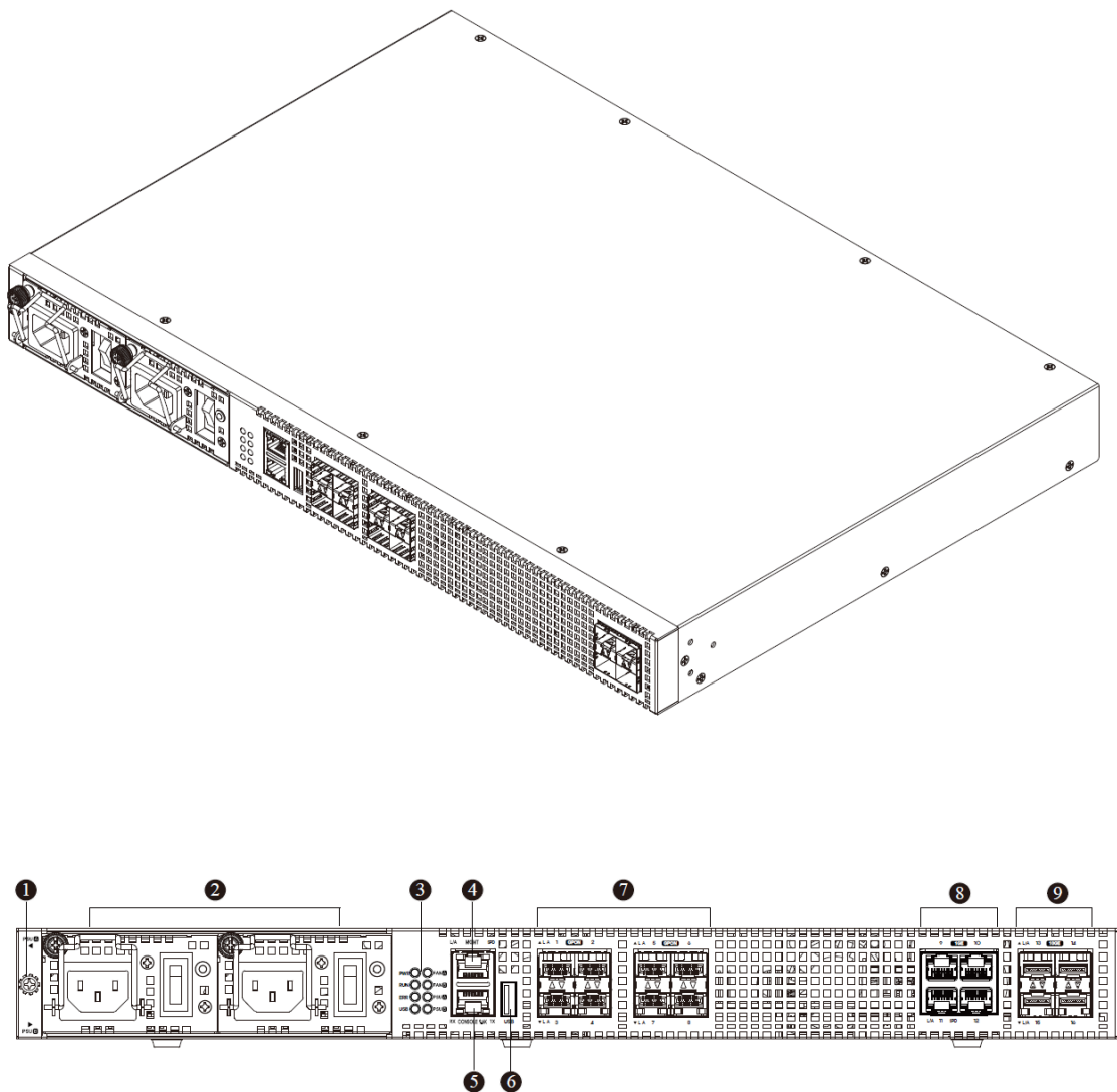
Figure 1 Front View of V5808
