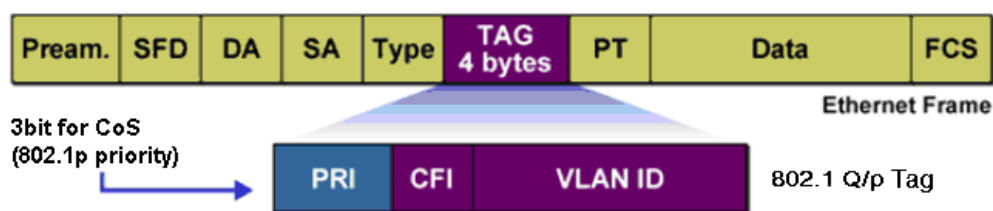
Figure 9-2 802.1Q frame
