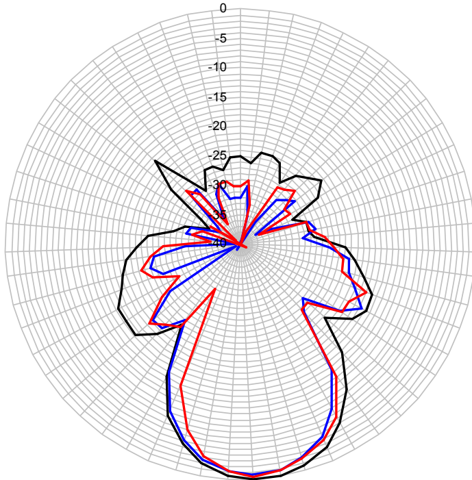
Radiation pattern envelope (RPE) V - polarization
