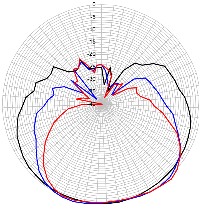
Radiation pattern envelope (RPE) V - polarization
